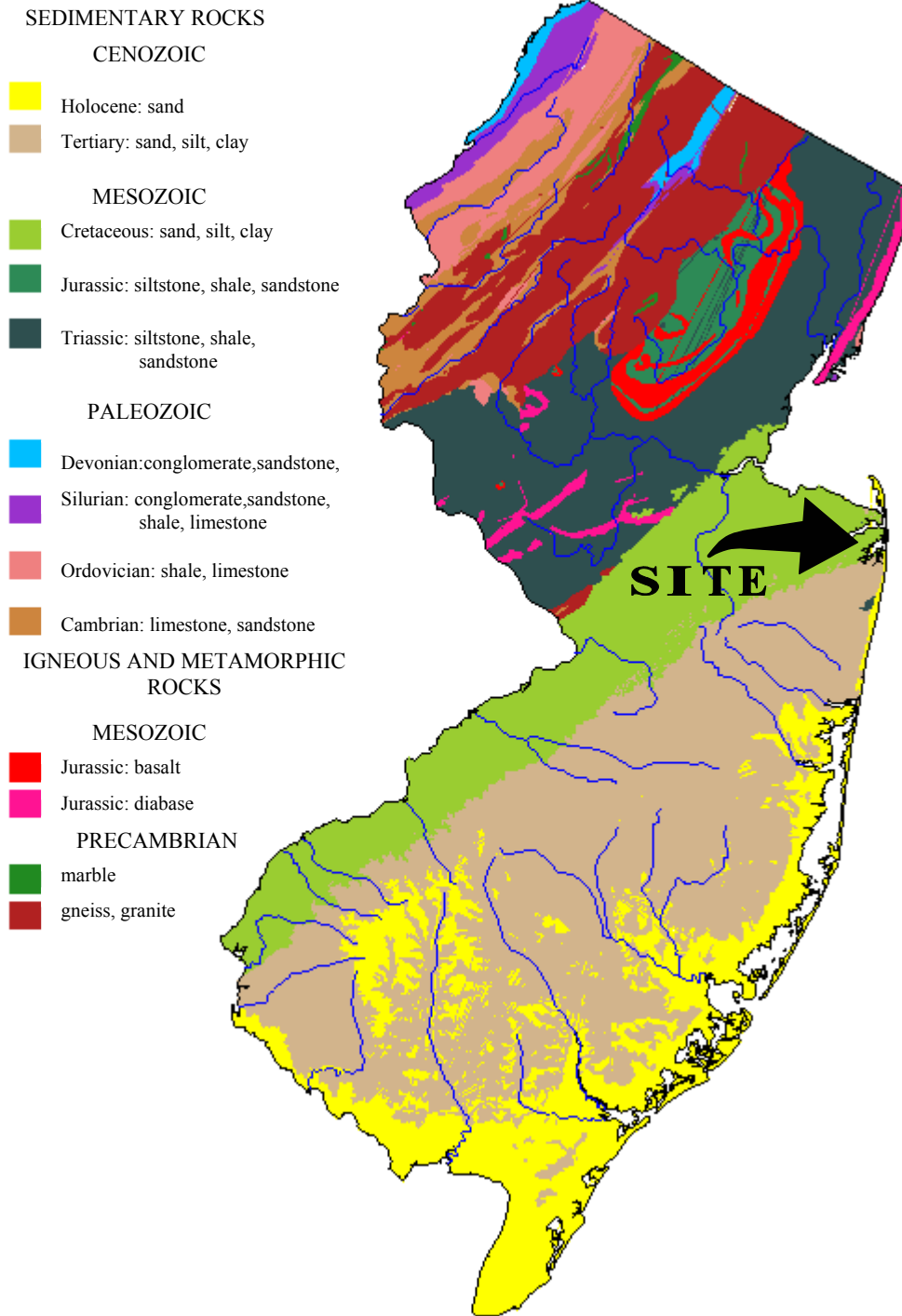
Figure 2-4 Geologic Map of New Jersey M-5 Landfill Site Fort Monmouth, New Jersey
