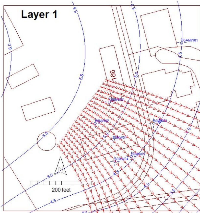
Parent MODFLOW Model
