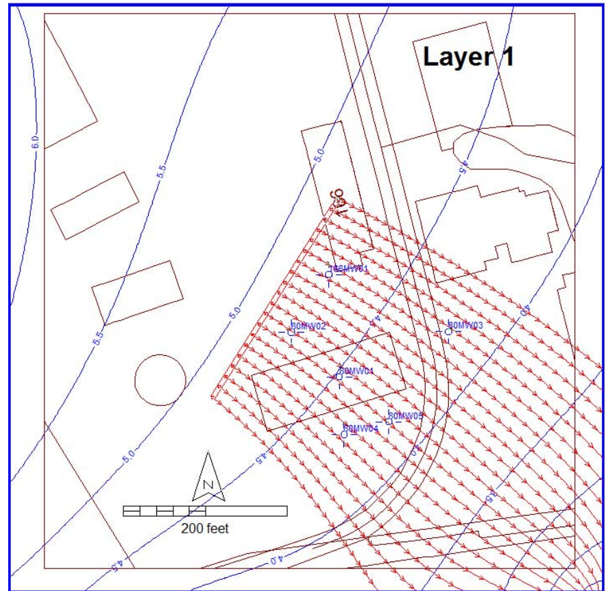
80-166 TMR MODFLOW Model
