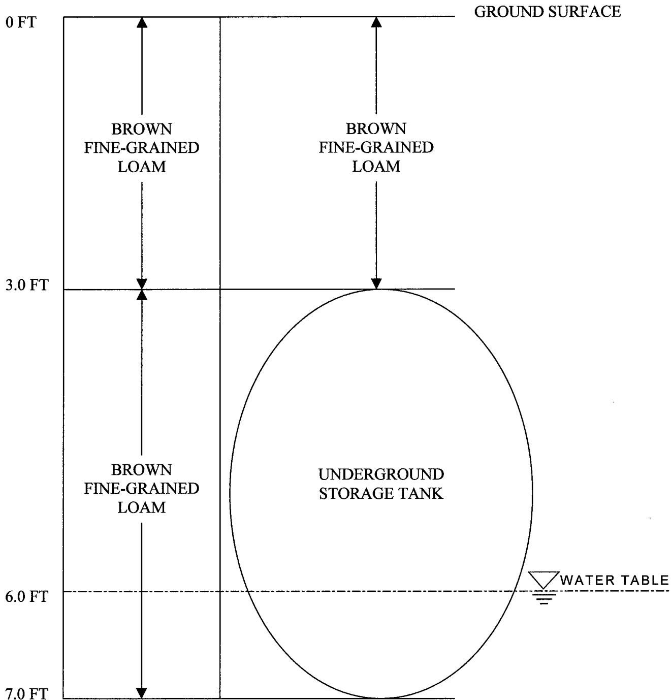
FIGURE 3 CROSS SECTIONAL VIEW BUILDING 276 FORT MONMOUTH ARMY BASE MONMOUTH COUNTY, NJ
