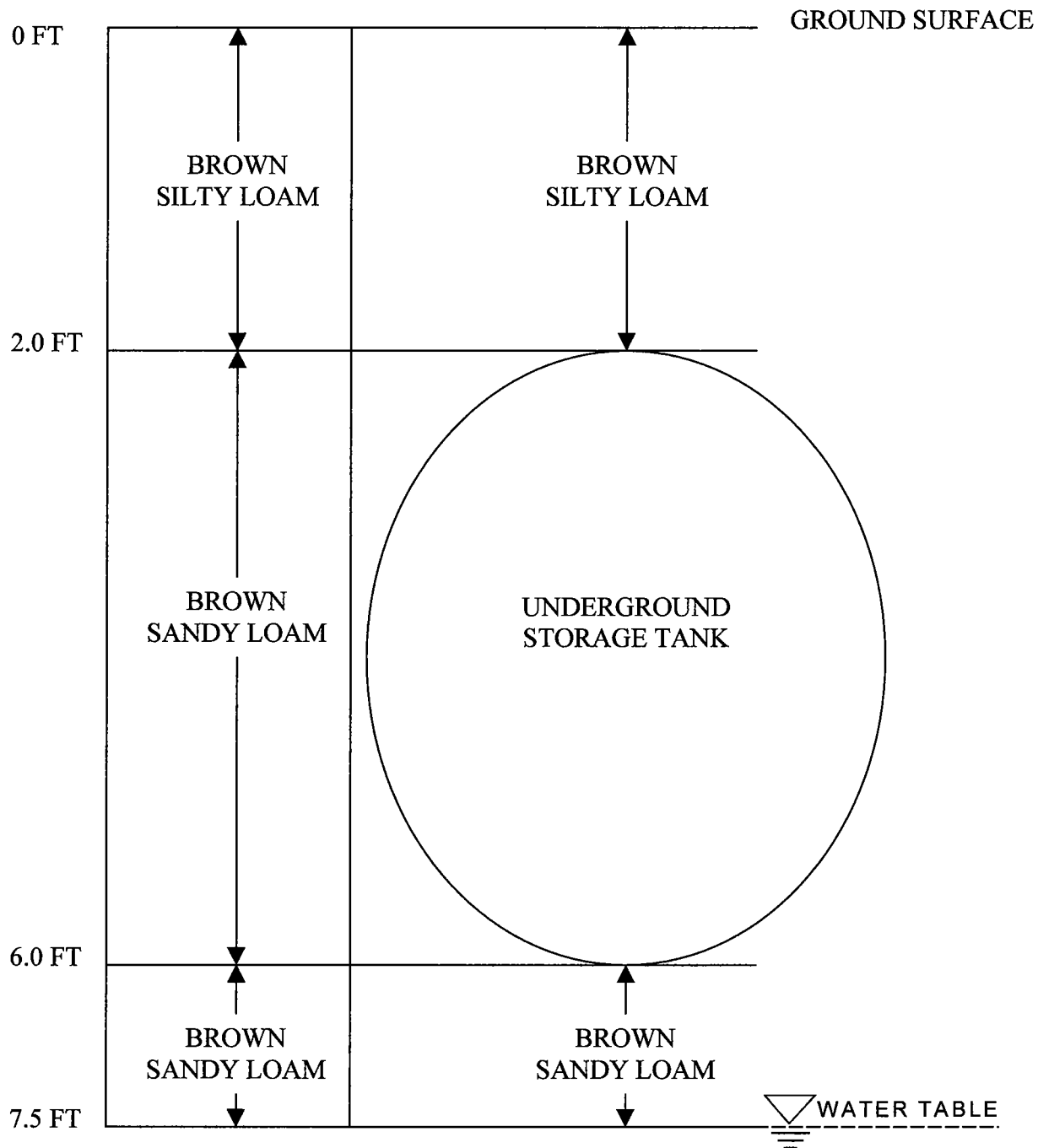
FIGURE 3 CROSS SECTIONAL VIEW BUILDING 752 FORT MONMOUTH ARMY BASE MONMOUTH COUNTY, NJ
