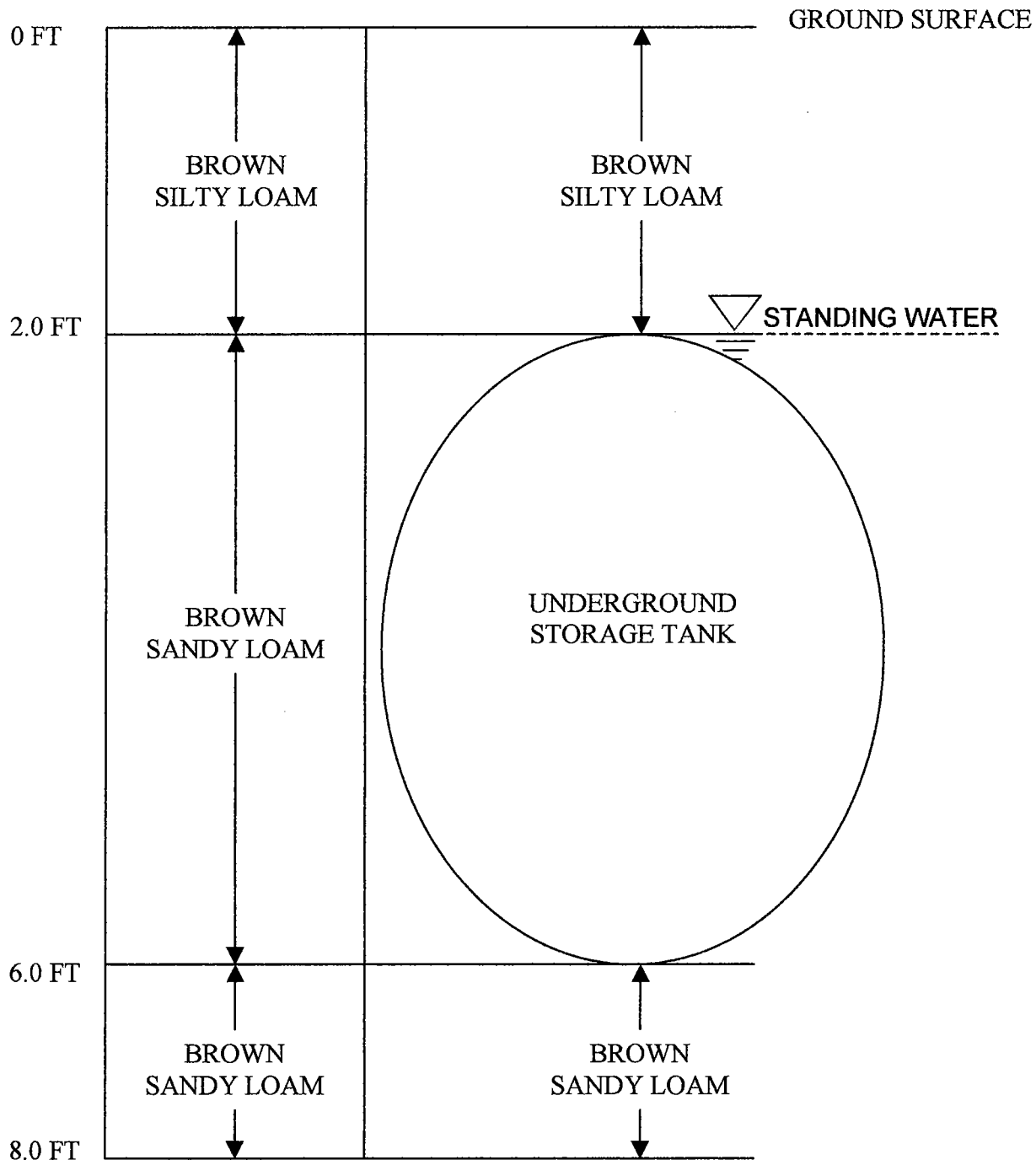
FIGURE 3 CROSS SECTIONAL VIEW BUILDING 875 FORT MONMOUTH ARMY BASE MONMOUTH COUNTY, NJ
