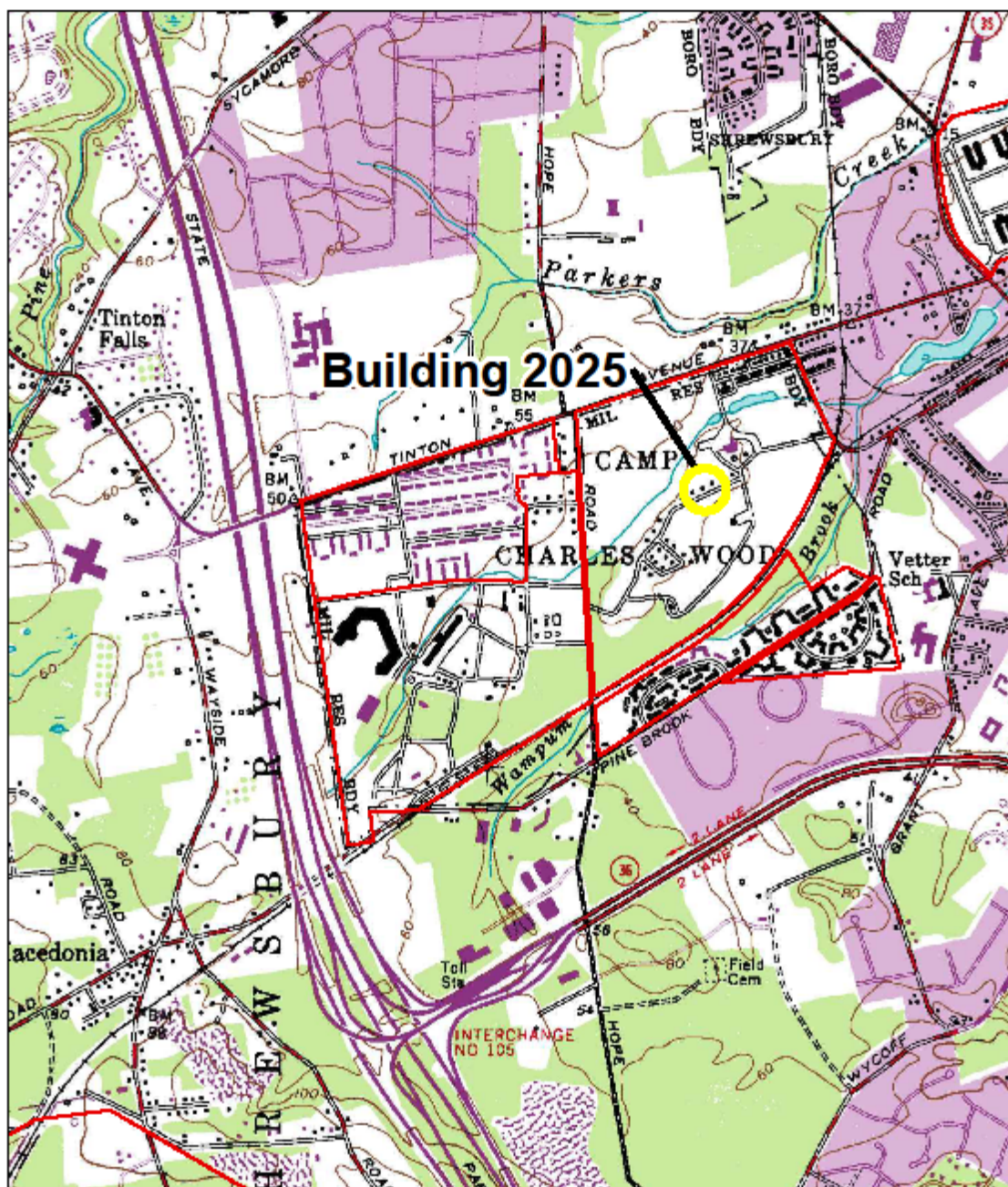
Figure 1 Location Map Building 2025, Charles Wood Fort Monmouth, NJ Date: 1/2011 UST Registration # 192486-6 UST Discharge # NA
